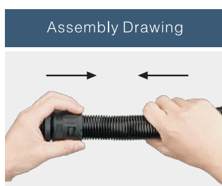
Assemble: Insert the flexible directly into the connector
