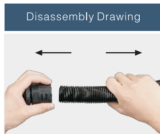
Disassemble: Tighten the connector to left, turn and pull the flexible tube to right
