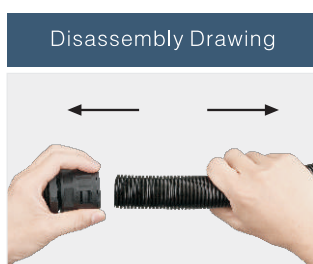
Disassemble: Tighten the connector to left, turn and pull the flexible tube to right
